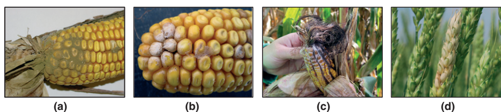
Fig. 1. Disease symptoms caused by (a) Aspergillus flavus (Aspergillus ear rot of maize), (b) Fusarium verticillioides (Fusarium ear rot of maize), (c) Fusarium graminearum (Gibberella ear rot of maize), and (d) F. graminearum (head scab of wheat/barley).
