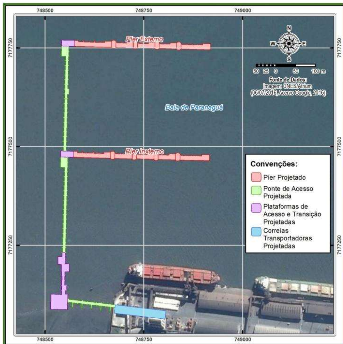
Figura 3.4 –Pier F
