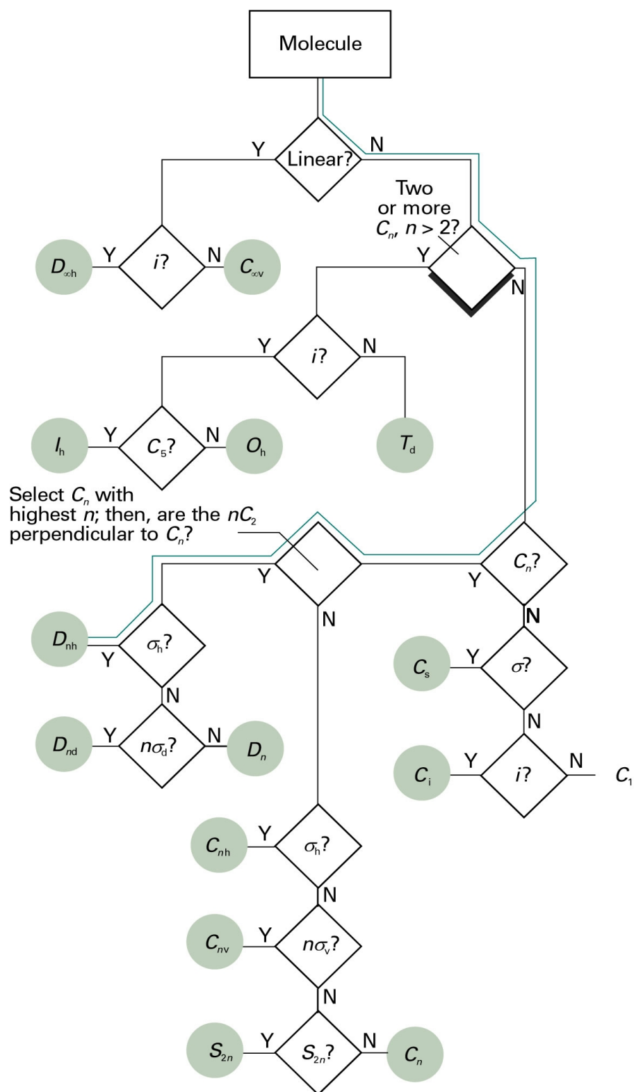
Fig. 12.7 A flow diagram for determining the point group of a molecule. Start at the top and answer the question posed in each diamond (Y = yes, N = no).
