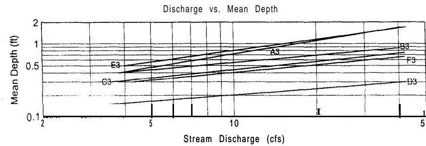
Fig. 11. Hydraulic geometry relations for selected stream types of uniform size.
