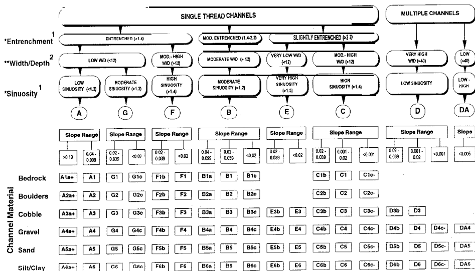
Fig. 5. Key to classification of natural rivers.
